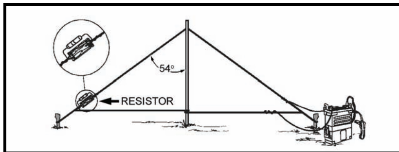
Figure 6-22. High frequency antenna, half-rhombic type.
