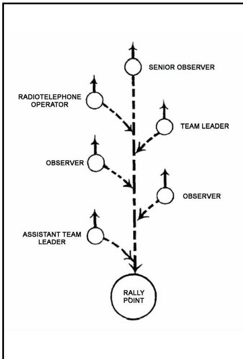
Figure H-2. Break contact front, left and right (Australian peel).
