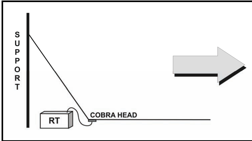
Figure 6-10. Unidirectional antenna pattern.
