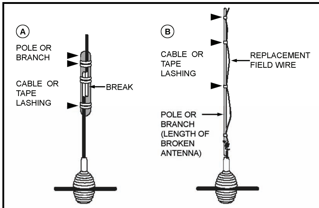
Figure 6-19. Repair procedure, whip antenna.
