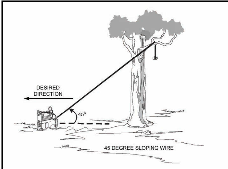
Figure 6-17. Sloping wire antenna.
