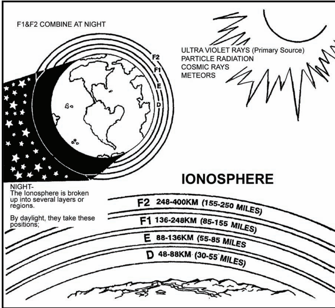
Figure 6-8. Structure of ionosphere.
