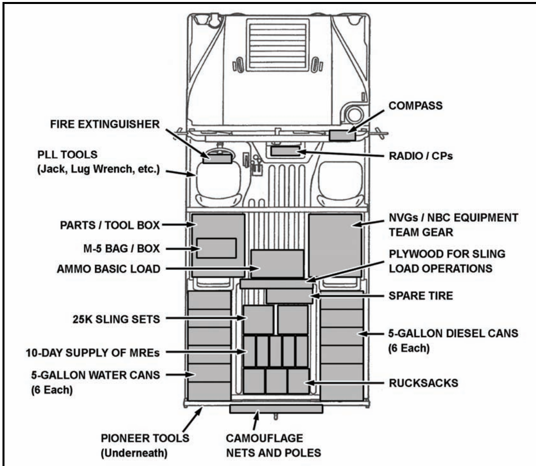
Figure 5-15. Example vehicle load configuration.
