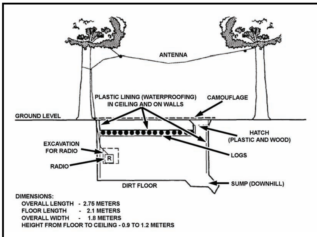
Figure 4-8. Example hide site.
