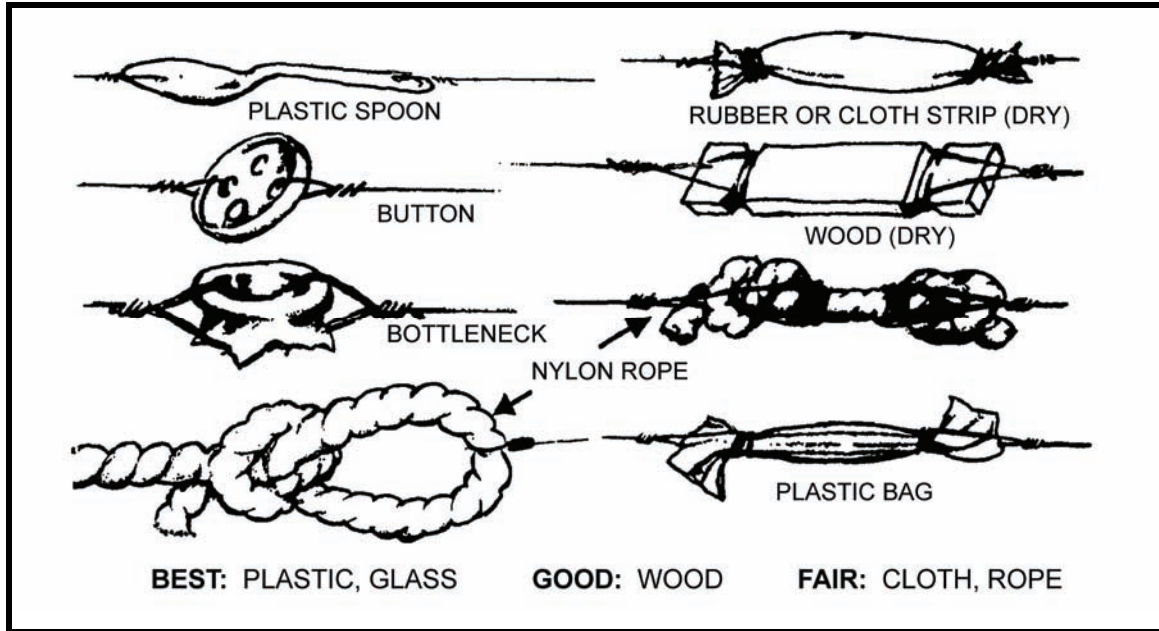
Figure 6-20. Expedient insulators.
