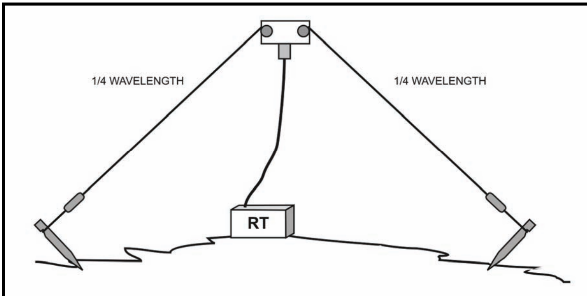
Figure 6-15. Inverted "V" antenna.
