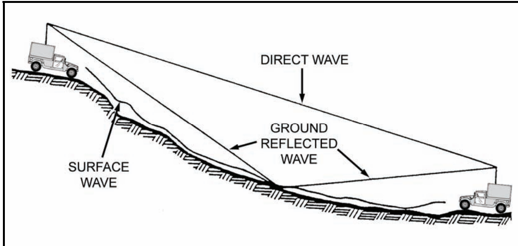
Figure 6-7. Components of ground wave.
