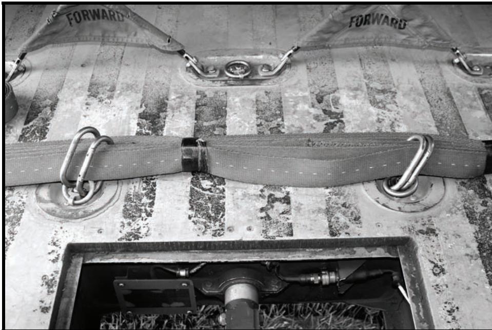
Figure 5-4. Rigging of snap links.
