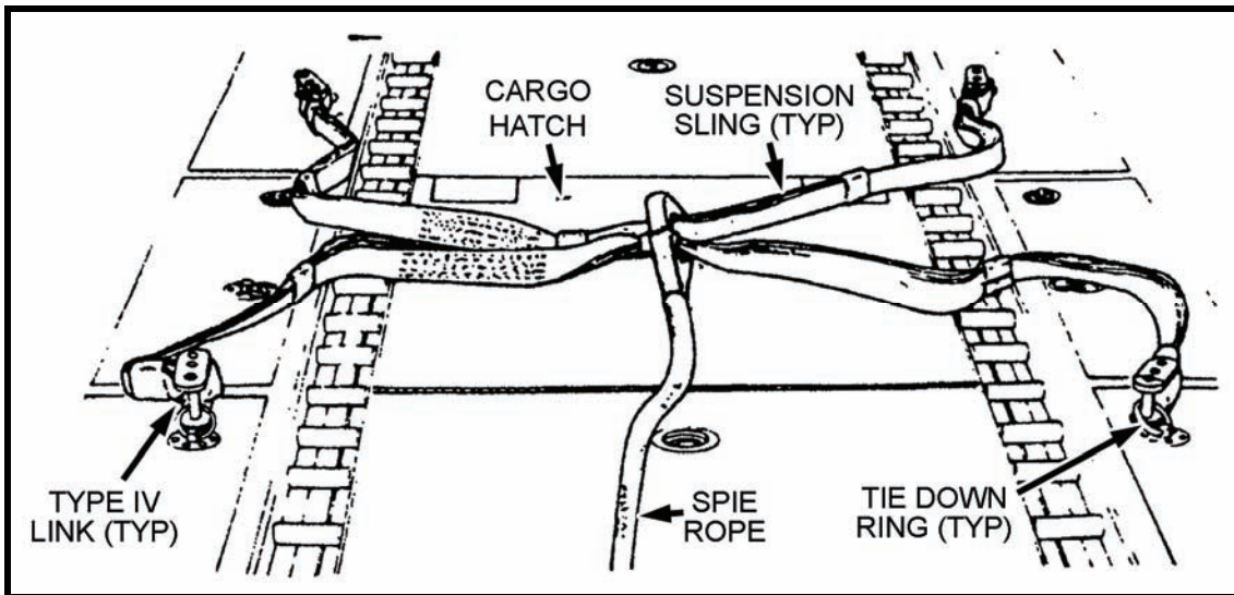
Figure 5-8. SPIES rigging procedures for CH-46 or CH-47.
