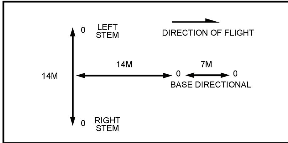
Figure 5-12. Marking procedures for landing and pickup zones.
