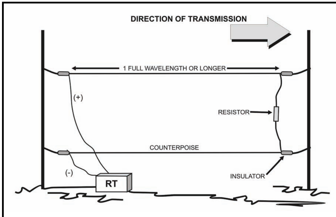
Figure 6-16. Long-wire antenna.
