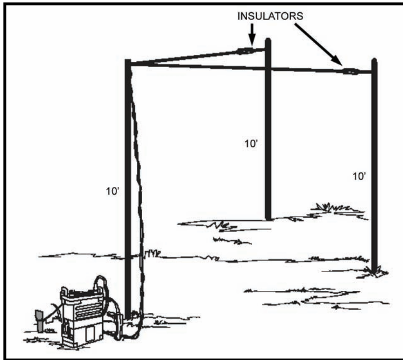
Figure 6-23. High frequency antenna, "V" type.
