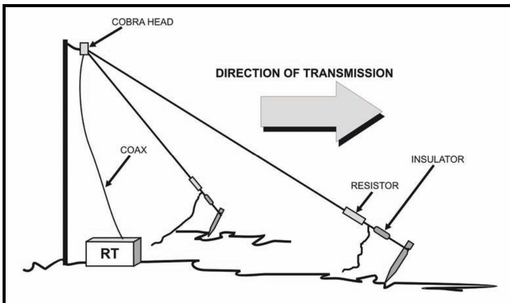
Figure 6-18. Terminated sloping "V" antenna.
