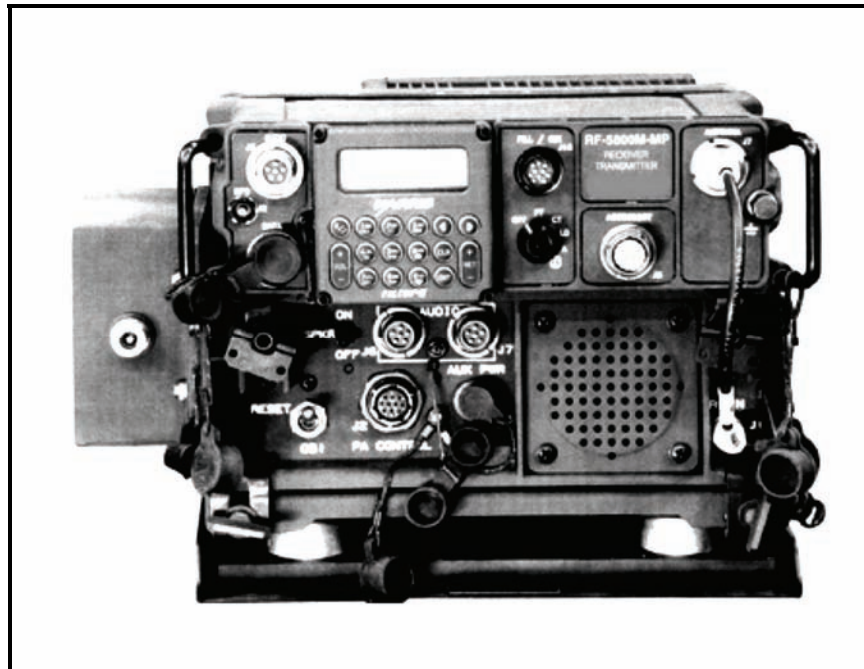
Figure 6-2. AN/PRC-150(C) in vehicular AN/VRC-104 (V)3 configuration.
